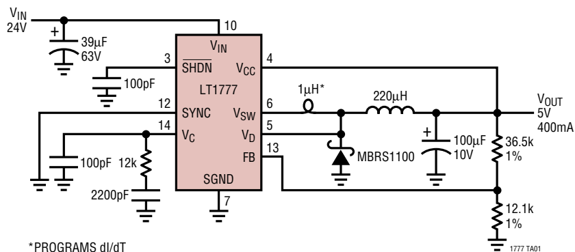
Low Noise 5V Step-Down Supply
