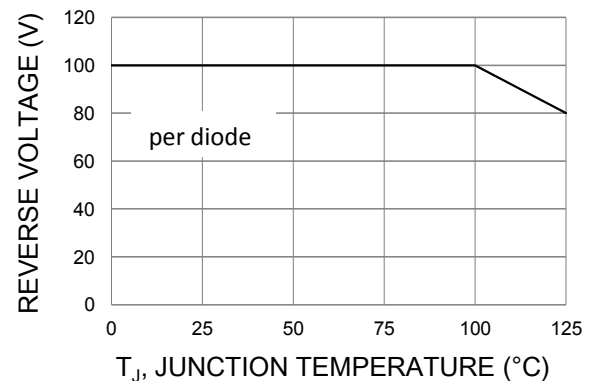
Fig.4 Operating Temperature Derating Curve
