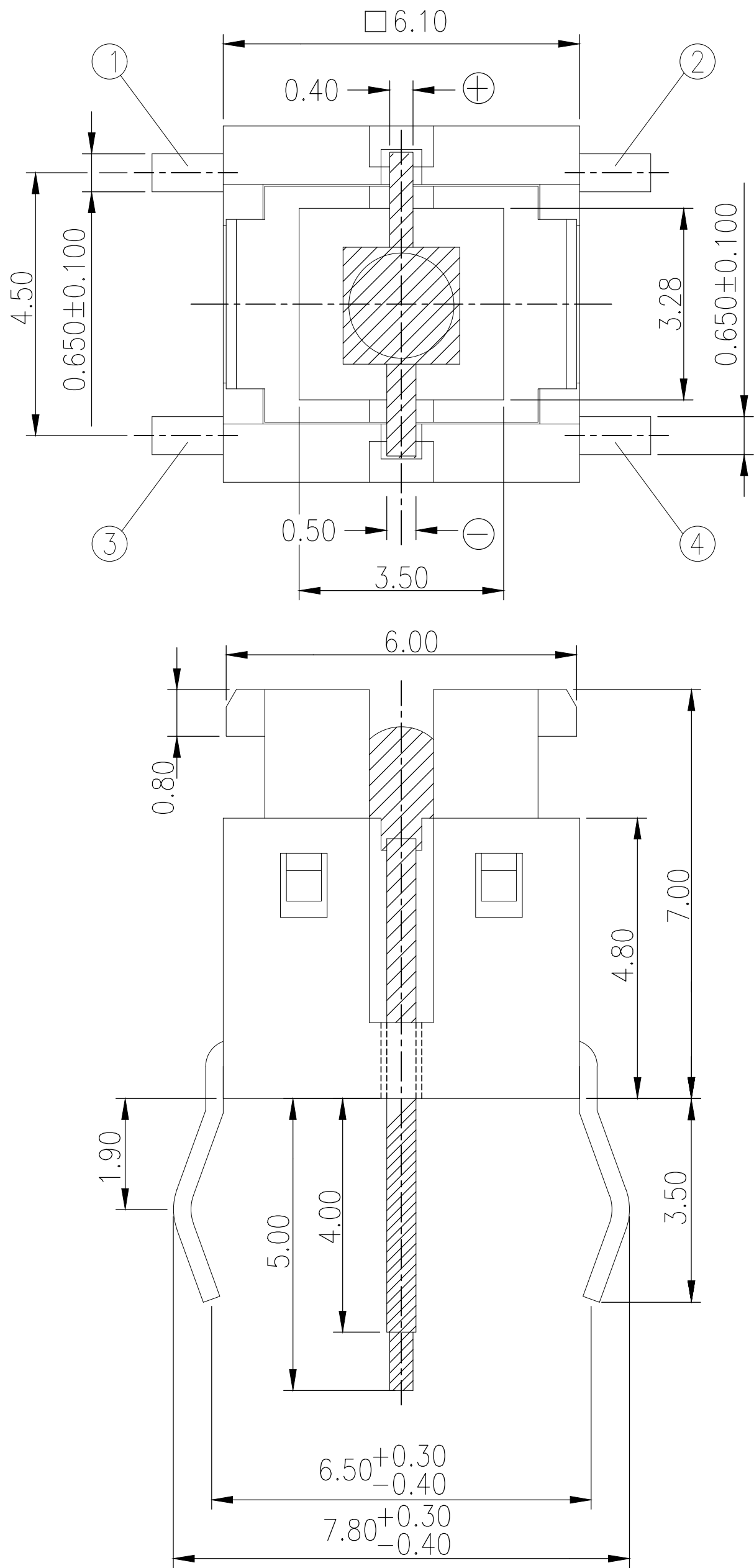
HIGH INTENSITY LED PROFILE
