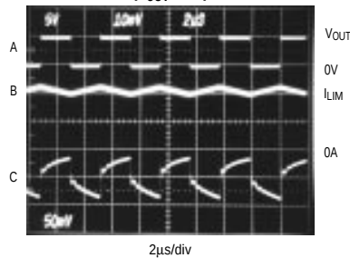
HEAVY-LOAD SWITCHING WAVEFORMS ( V_{OUT} = 5\text{V} )
