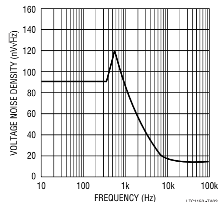
Noise Spectrum
