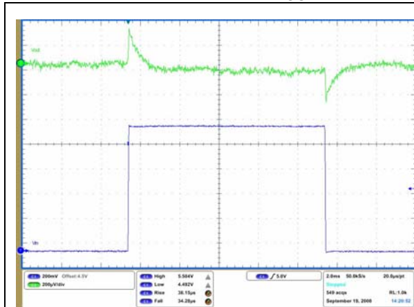
Figure 16. Line transient ( V_{OUT} = 3.3\text{ V} )
