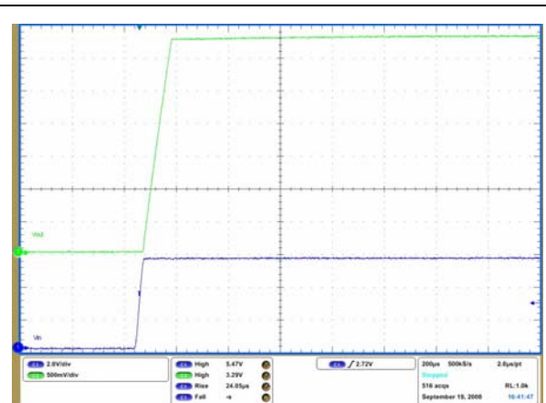
Figure 19. Start-up transient
