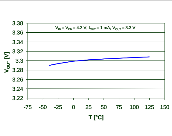
Figure 5. V_{OUT} vs. temperature ( V_{OUT} = 3.3 V )
