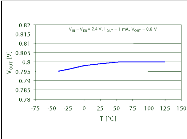
Figure 4. V_{OUT} vs. temperature ( V_{OUT} = 0.8 V )
