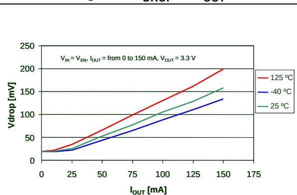
Figure 9. V_{DROP} vs. I_{OUT}
