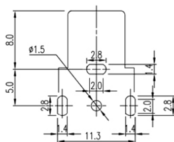
T:1.6 Dimensions of PC board holes Tolerance : ±0.05(Printed-bottom view)
