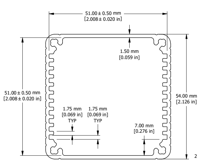
EXTRUSION
