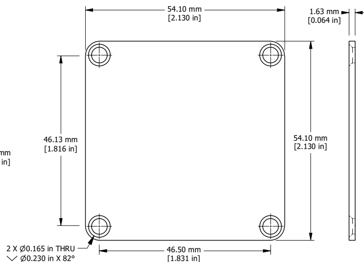
END PLATE
