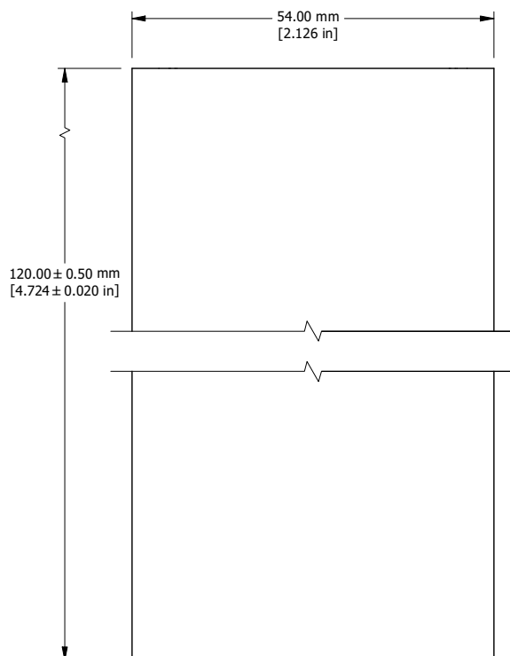
EXTRUSION
