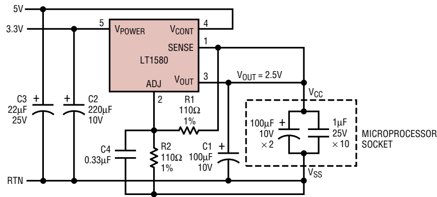
2.5V/6A Regulator
