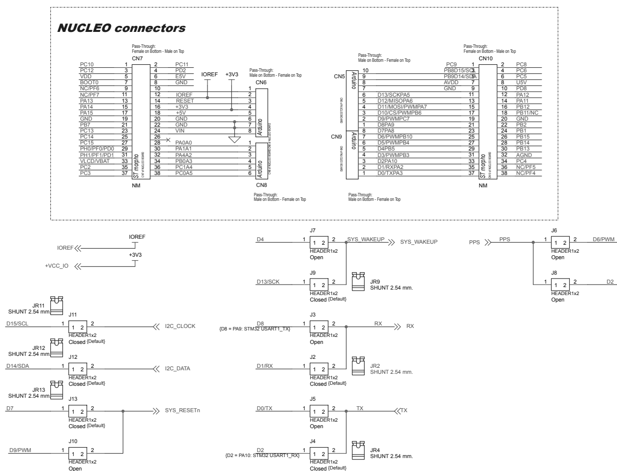
Figure 3. X-NUCLEO-GNSS1A1 circuit schematic (3 of 3)
