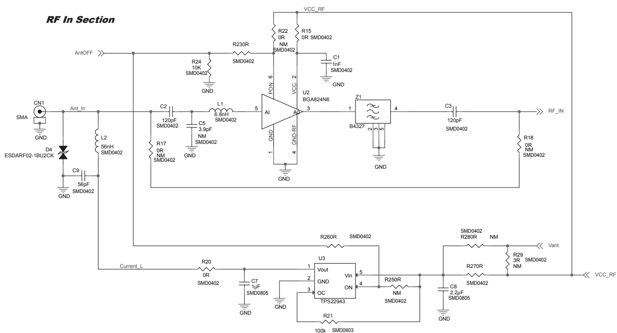
Figure 3. X-NUCLEO-GNSS1A1 circuit schematic (3 of 3)
