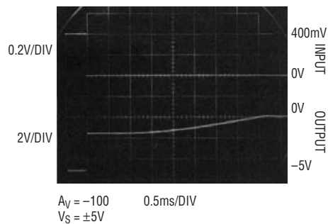
Overload Recovery
