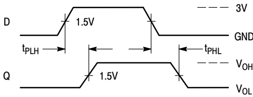
Figure 3. Switching Waveform
