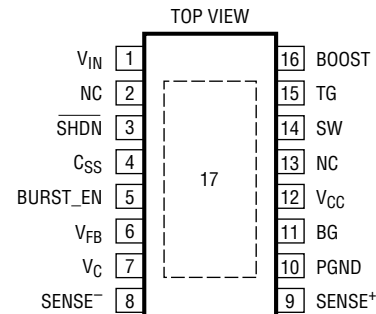
FE PACKAGE 16-LEAD PLASTIC TSSOP T_{JMAX} = 125^{\circ}\text{C} , \theta_{JA} = 40^{\circ}\text{C/W} , \theta_{JC} = 10^{\circ}\text{C/W} EXPOSED PAD (PIN 17) IS SGND MUST BE SOLDERED TO PCB
