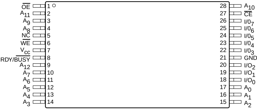
TSOP Top View (8mm x 13.4mm) (T13, H13)
