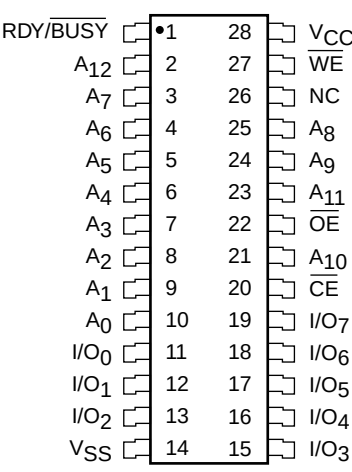
SOIC Package (J, W) (K, X)
