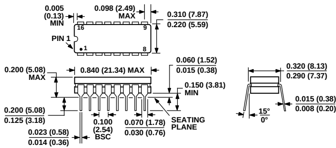
Figure 22. 16-Lead Ceramic Dual In-Line Package [CERDIP]
