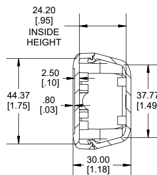
SECTION B-B END VIEW
