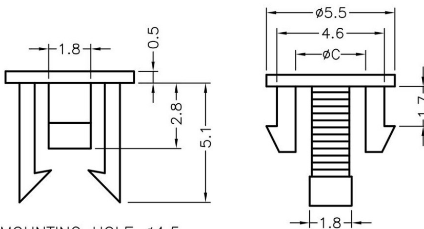
MOUNTING HOLE \phi 4.5 THICKNESS 1.6
