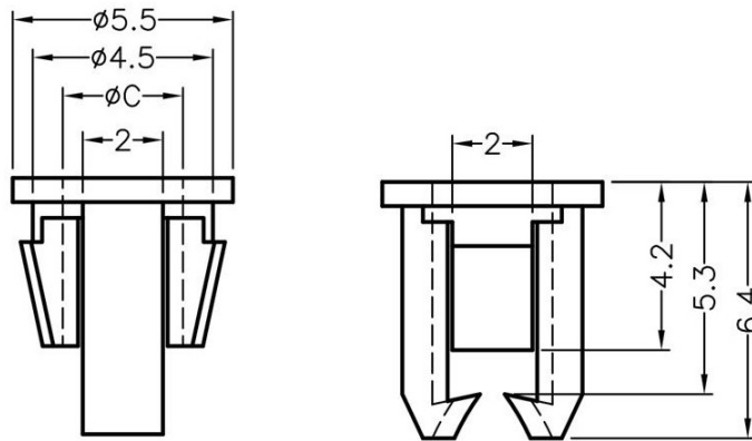
MOUNTING HOLE \phi 4.5 THICKNESS 0.8
