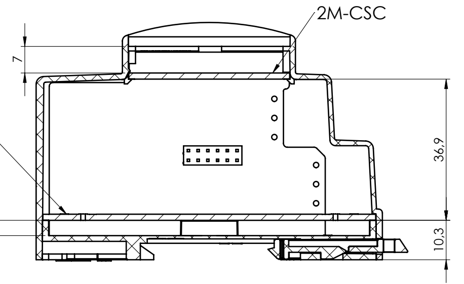
PCB-C assembly
