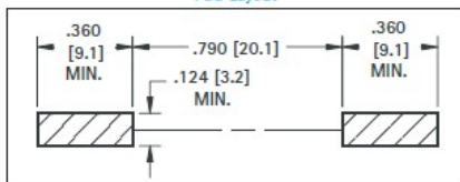
Pad Layout
