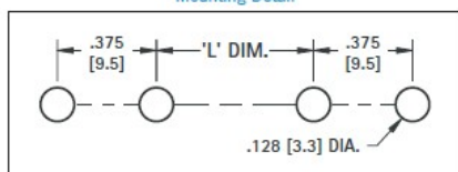
Mounting Detail
