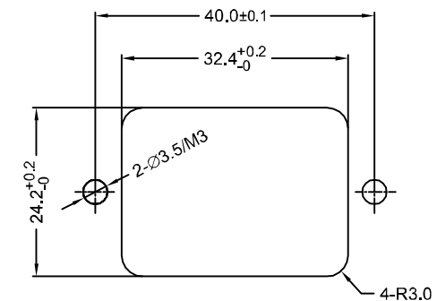
PANEL CUT-OUT
