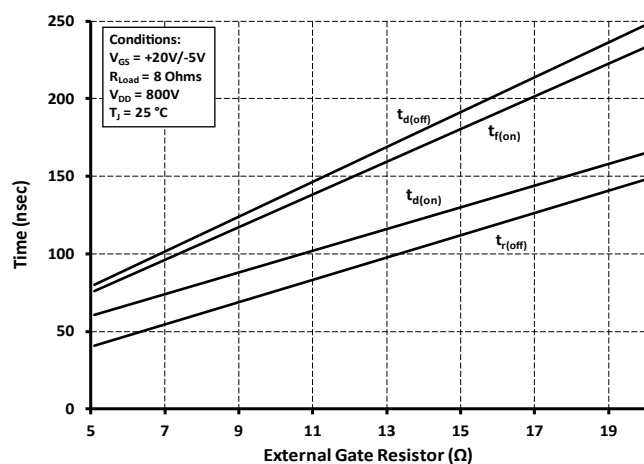
Figure 17. Timing vs. R_{G(\text{ext})}
