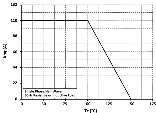
Figure 12. Forward derating curve of reverse diode
