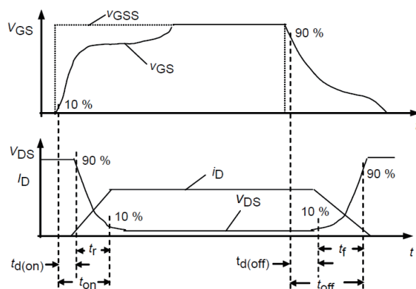
Figure 18. Resistive Switching Time Description
