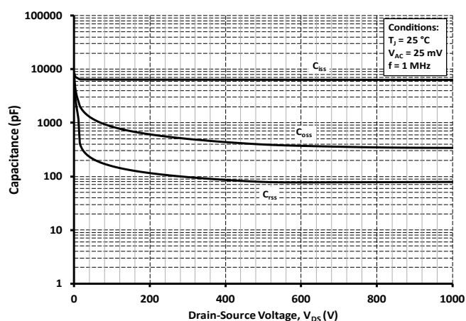
Figure 10. Capacitances vs. Drain-Source Voltage (0 - 1 kV)
