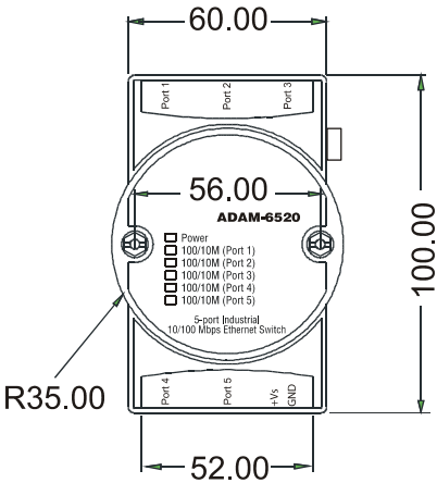
Figure 2.2: Front Panel
