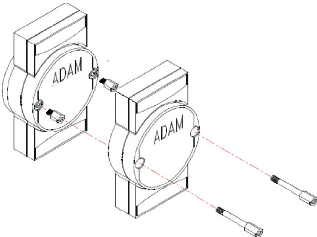
Figure 2.6: Piggyback Stacking
