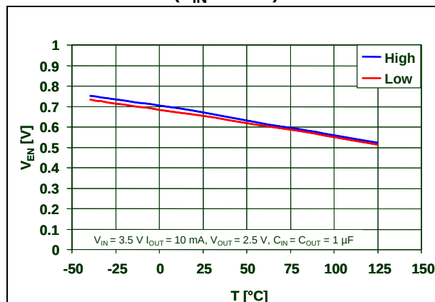
Figure 24. Enable voltage vs. temperature ( V_{IN} = 3.5 V)
