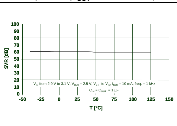
Figure 19. Supply voltage rejection vs. temperature ( V_{OUT} = 2.5\text{ V} , f = 1\text{ kHz} )
