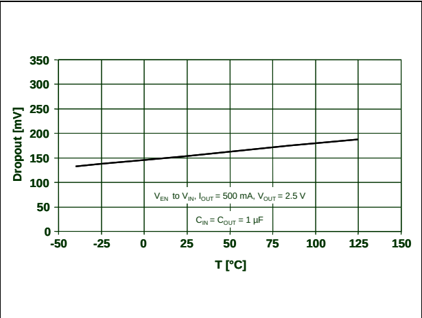
Figure 7. Dropout voltage vs. temperature ( V_{OUT} = 2.5\text{ V} )
