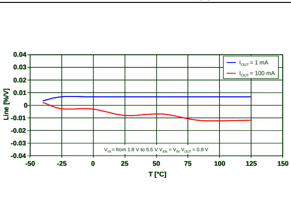
Figure 15. Line regulation ( V_{OUT} = 0.8\text{ V} )
