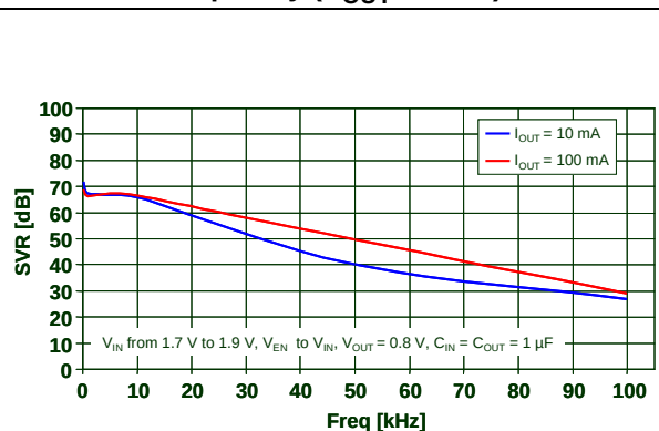
Figure 21. Supply voltage rejection vs. frequency ( V_{OUT} = 0.8 V)
