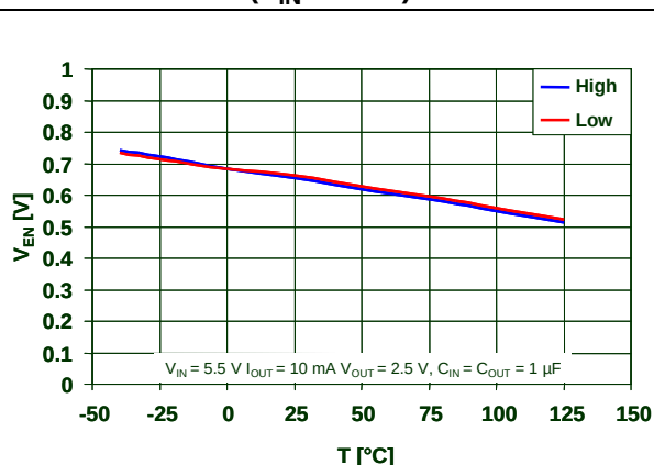
Figure 25. Enable voltage vs. temperature ( V_{IN} = 5.5 V)
