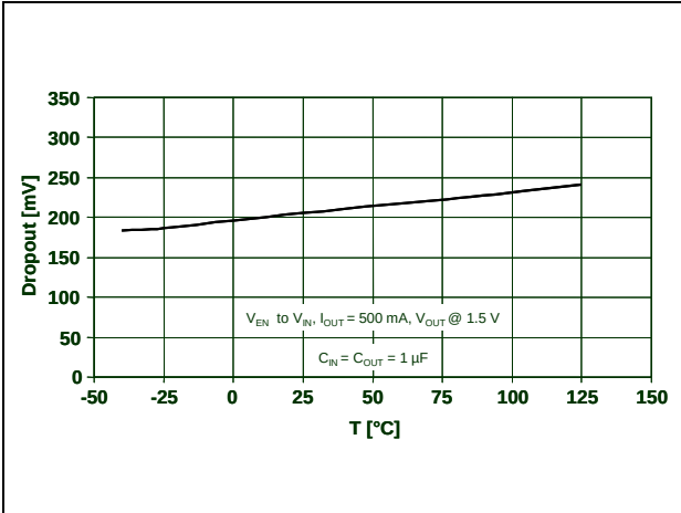
Figure 6. Dropout voltage vs. temperature ( V_{OUT} = 1.5\text{ V} )
