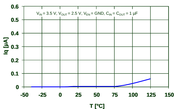
Figure 13. Quiescent current in OFF mode vs. temperature
