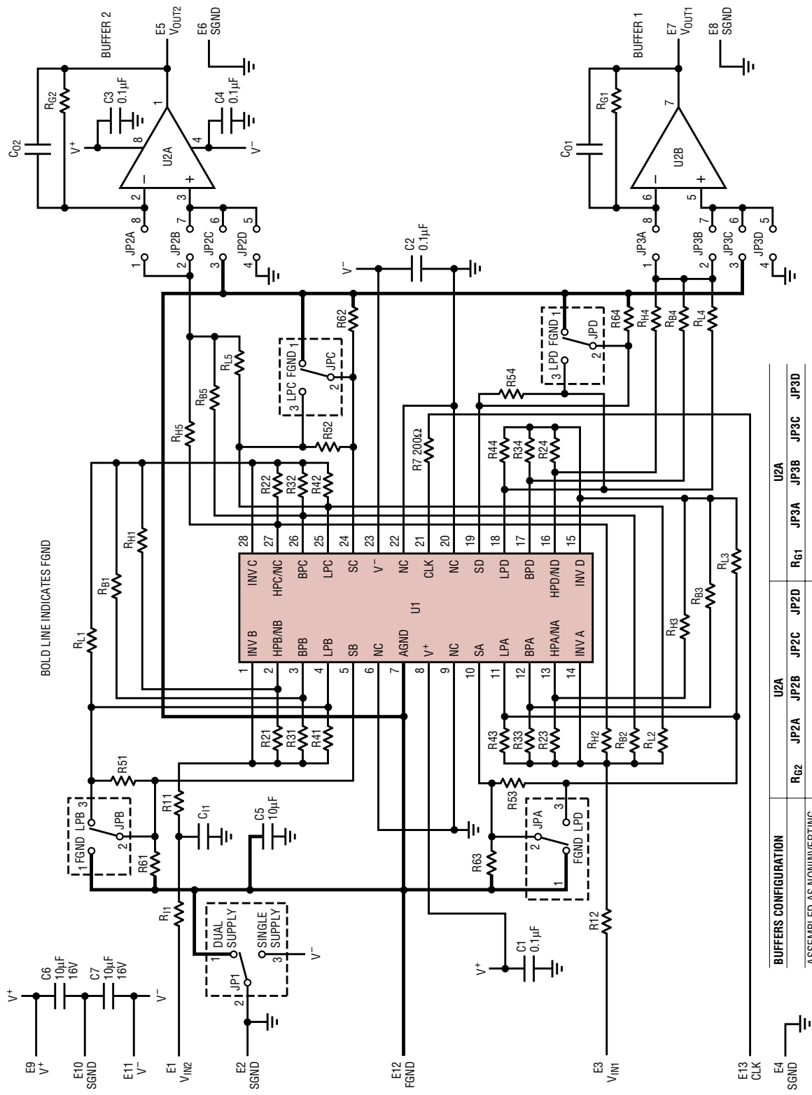
DC104 Schematic
