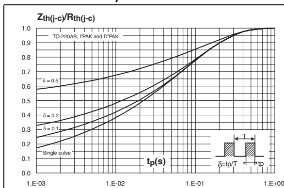
Figure 7. Relative variation of thermal impedance junction to case versus pulse duration (TO-220AB, D 2 PAK, I 2 PAK)
