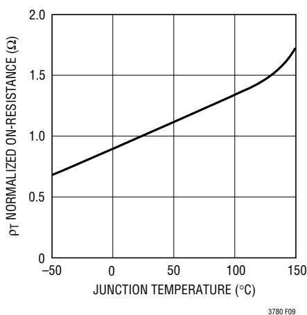
Figure 9. Normalized R_{DS(ON)} vs Temperature
