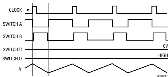
Figure 3. Buck Mode ( V_{IN} > V_{OUT} )
