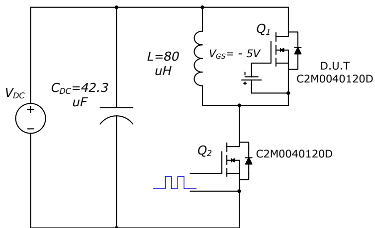
Figure 31. Body Diode Recovery Test Circuit
