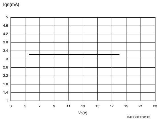
Figure 8. Current consumption vs. input voltage ( I_o = 75\text{ mA} )
