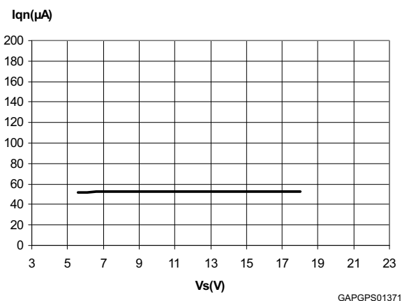
Figure 7. Current consumption vs. input voltage ( I_o = 0.1\text{mA} )
