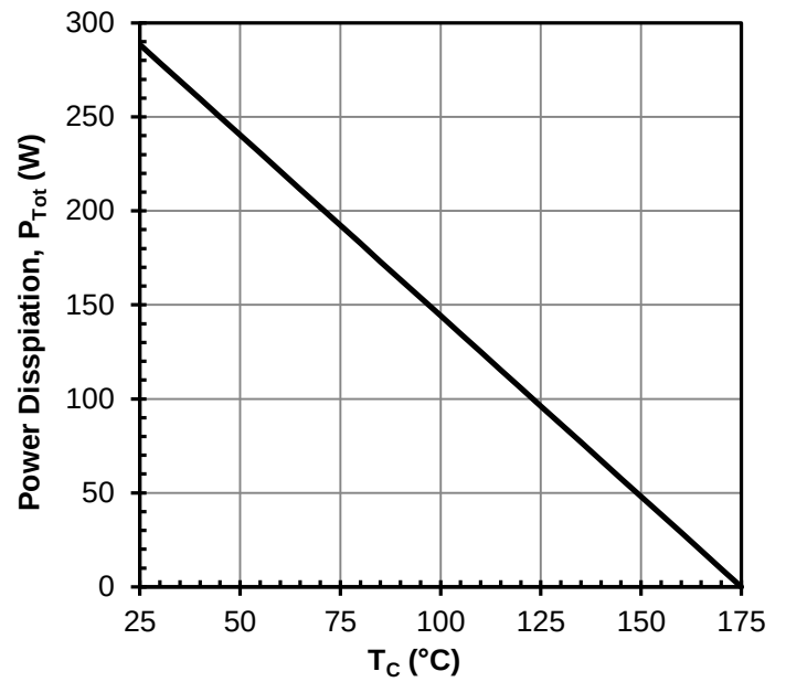
Figure 4 Power dissipation
