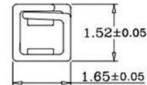
Section C-C
