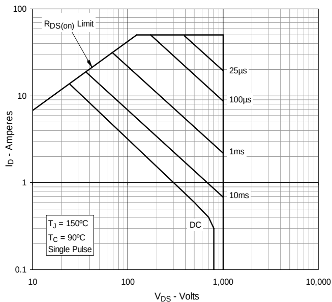
Fig. 14. Forward-Bias Safe Operating Area @ T_C = 90^\circ\text{C}
