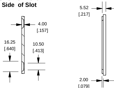
SECTION C-C Side of Slot
