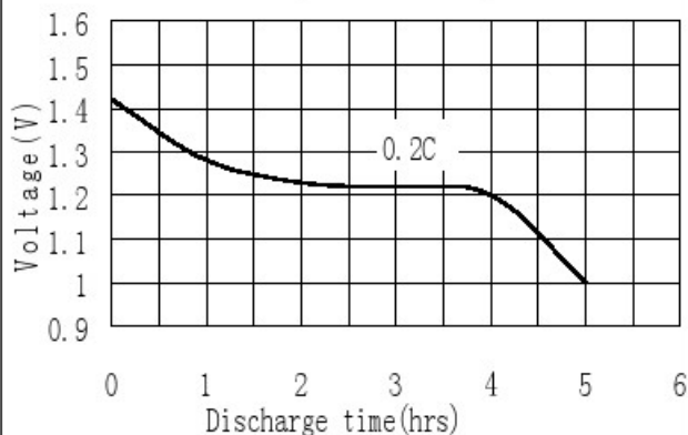
Discharge at low rate, 20°C
