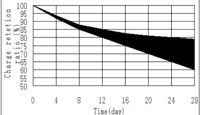
Selfdischarge at 20°C
