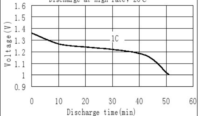
Discharge at high rate, 20°C
