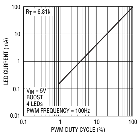
Figure 5. LED Current vs PWM Duty Cycle Wide Dimming Range (500:1)
