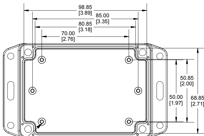
INSIDE BOX
