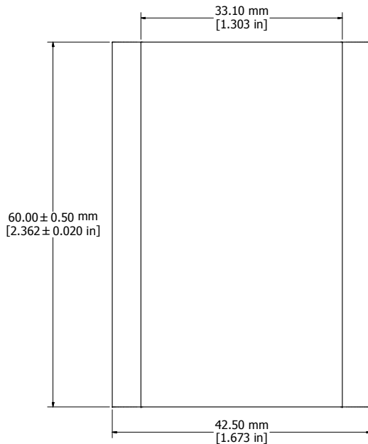
EXTRUSION PROFILE
