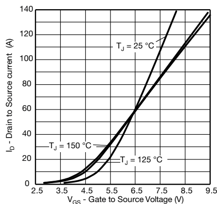
Fig. 8 - Typical MOSFET Transfer Characteristics
