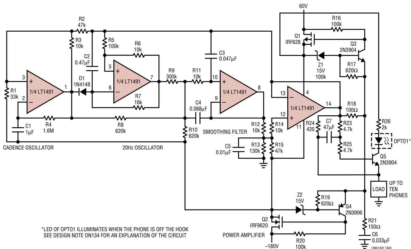
Ring-Tone Generator
