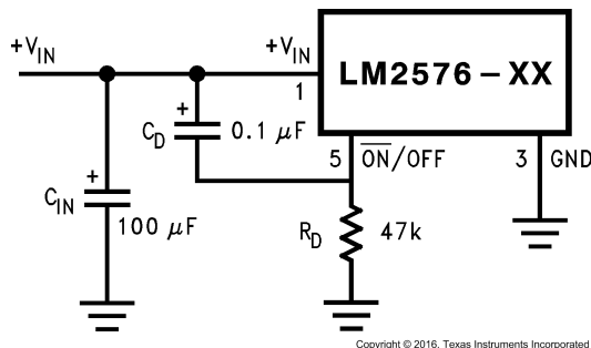
Figure 22. Delayed Start-Up
