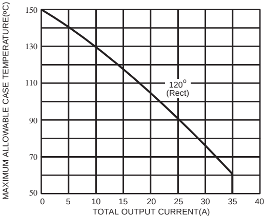
FIG. 5 - CURRET RATINGS CHARACTERISTICS
