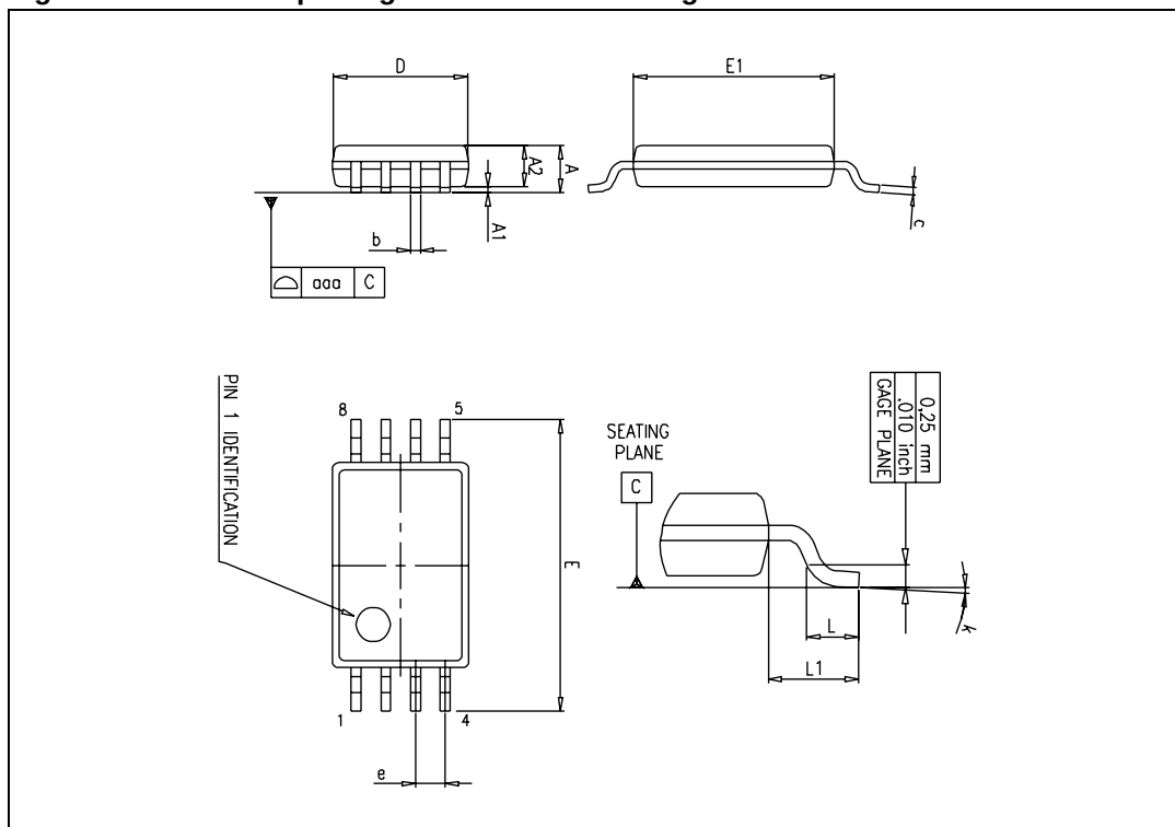
Figure 20. TSSOP8 package mechanical drawing
