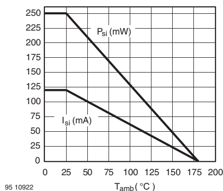
Figure 1. Derating diagram
