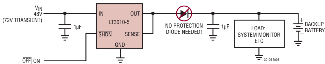
LT3010 Telecom Application
