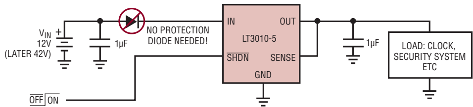
LT3010 Automotive Application
