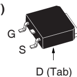
TO-252 (IXTY)
