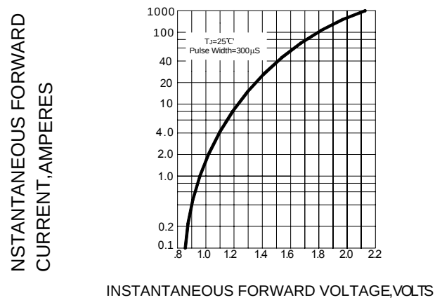
FIG.4 --TYPICAL FORWARD CHARACTERISTIC
