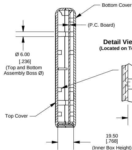
SECTION A-A (Side View Inside Assembly)
