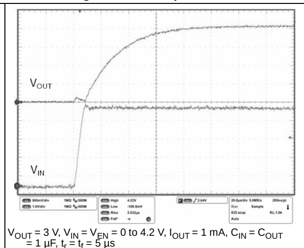
Figure 30. Startup transient
