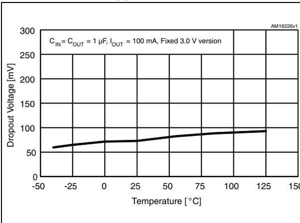
Figure 33. Dropout voltage vs. temperature ( I_{OUT} = 100 mA)
