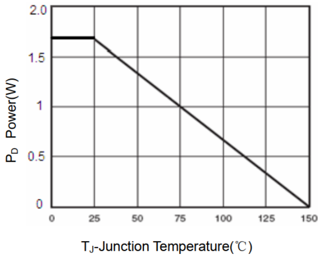
Figure 1. Power Dissipation
