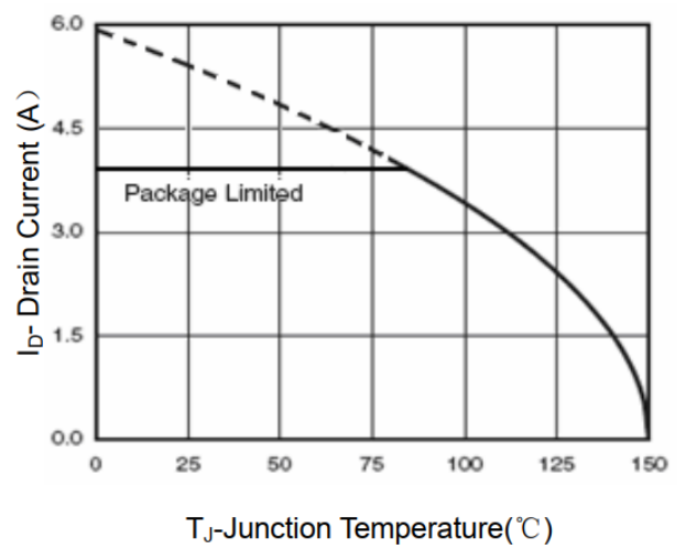
Figure 2. Drain Current
