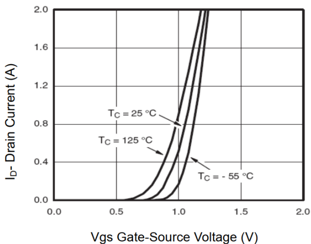
Figure 5. Transfer Characteristics
