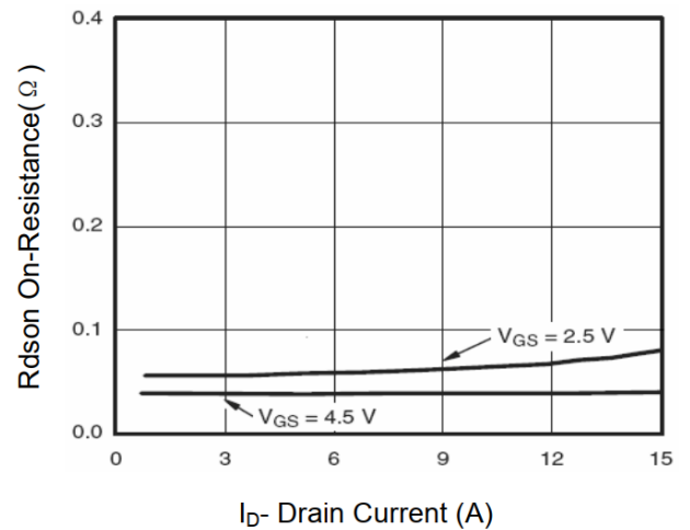
Figure 4. Drain-Source On-Resistance
