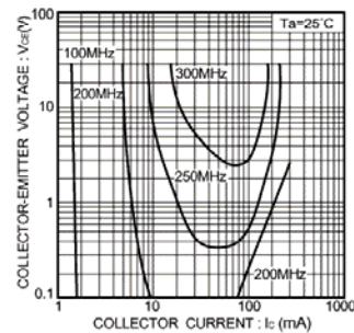
Fig.9 Gain bandwidth product
