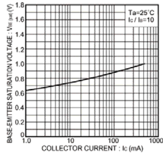
Fig.2 Base-emitter saturation voltage vs. collector current
