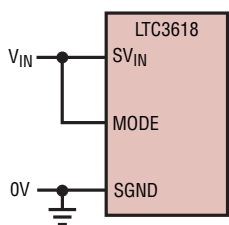
1a. Pulse-Skipping Mode
